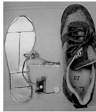
Figure 13. Shoe-Shaped Sensor
